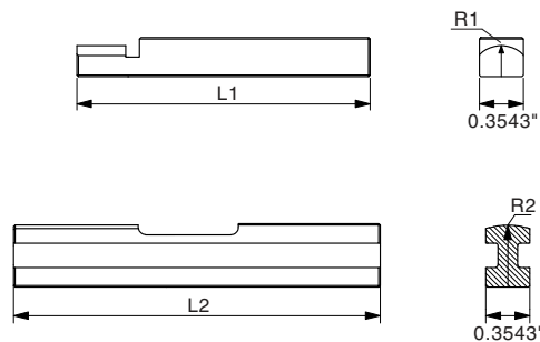
Cylindrical Jaws (E)
