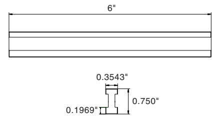
Flat Jaw (F)
