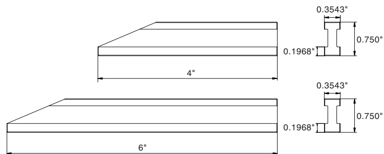
Jaw with Beveled Ends (H)
